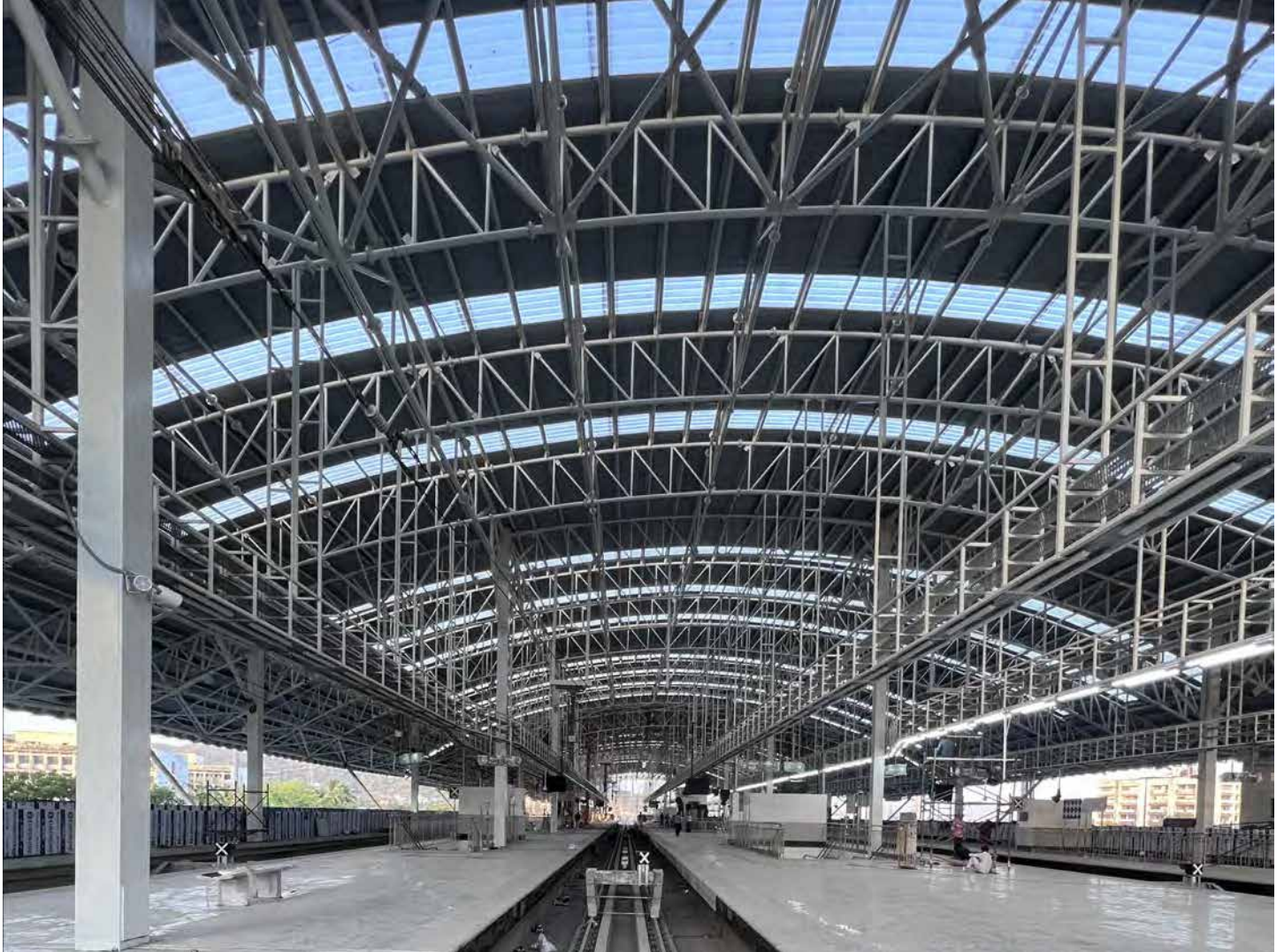
CBD Metro Station I - 800T I Supply , Fabrication and Erection
